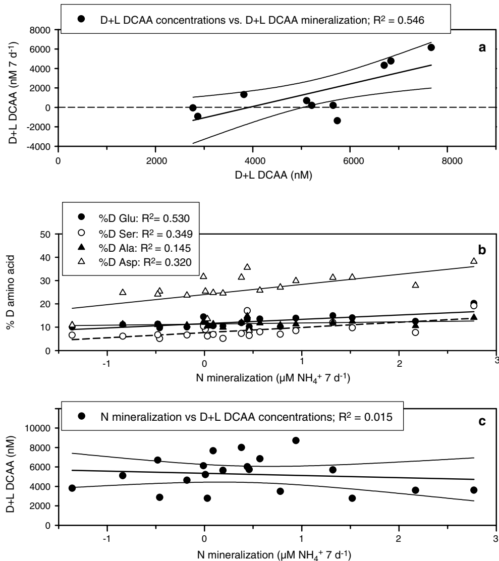
Fig. 4 Batch culture studies: correlations (linear regressions) between ambient concentrations and mineralization rates (uptake or release) of all D+L dissolved combined amino acids (DCAA) (a), between N mineralization
